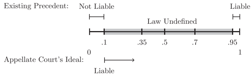
Figure 1: Numerical Example
